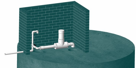
The Chlorinator ADEC is typically installed on top of the community's existing water storage tank.
